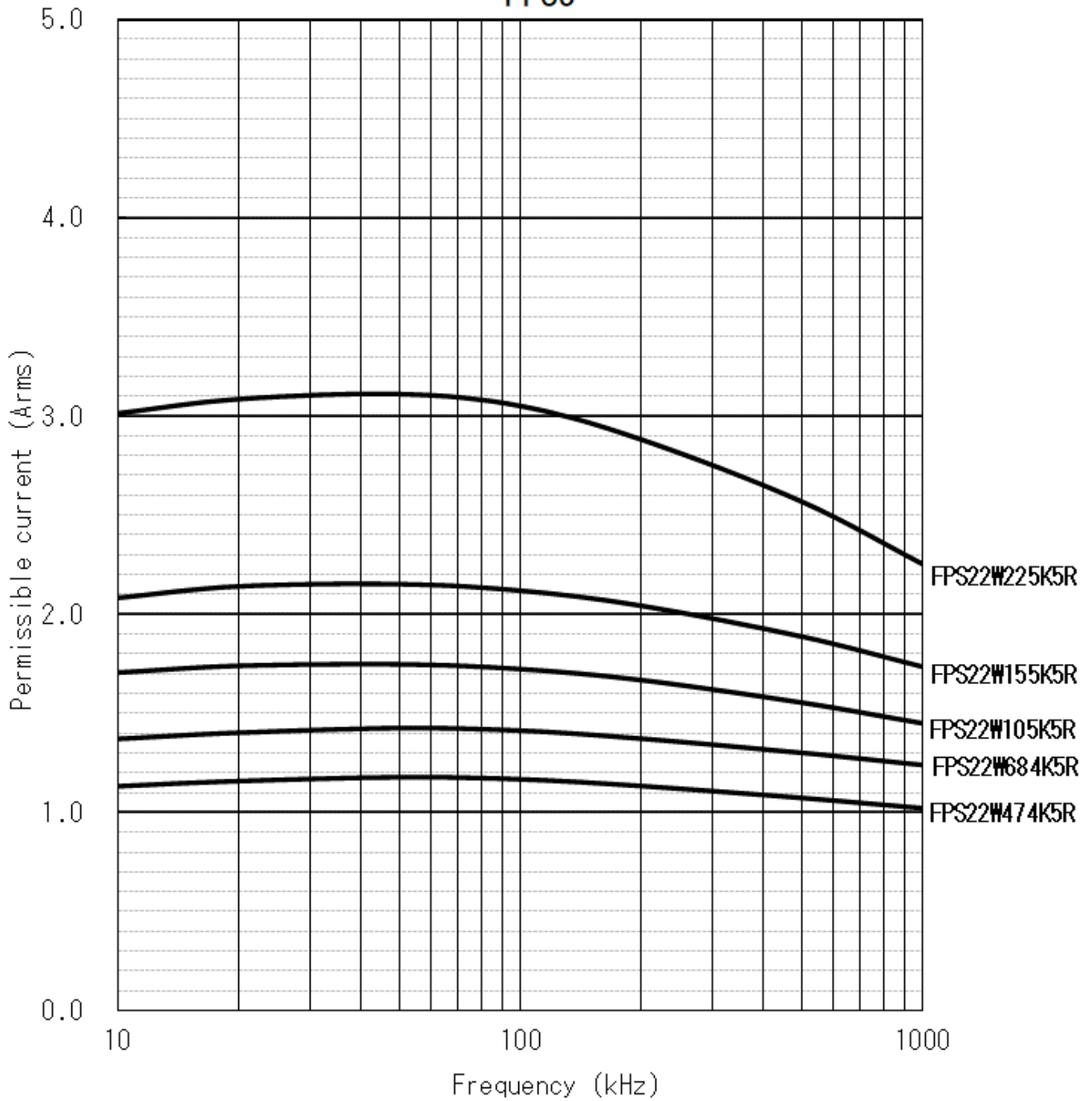
Permissible current (Effective value) VS Frequency FPS5
